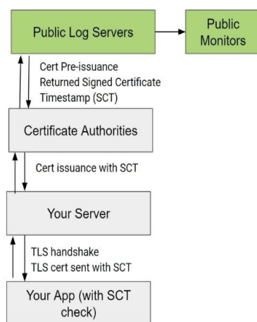
Figure 11: Blocking client-side MitM Attacks
