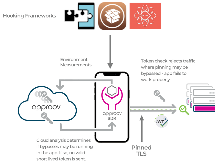
Figure 12: Blocking client-side MitM Attacks
